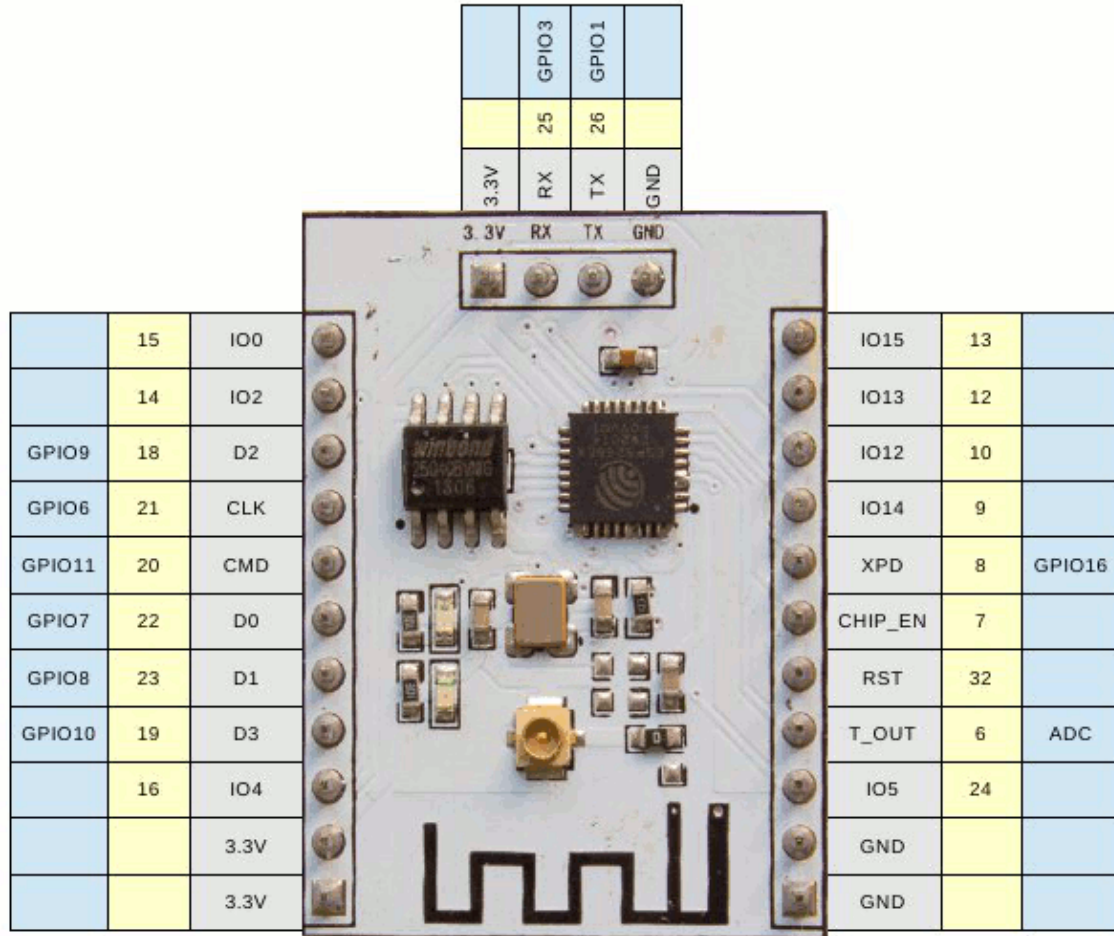
Text on ESP-201 board ESP8266 pin number Remarks ESP-201 pin reference v.0.1 (c) 2015 smarpl.com
